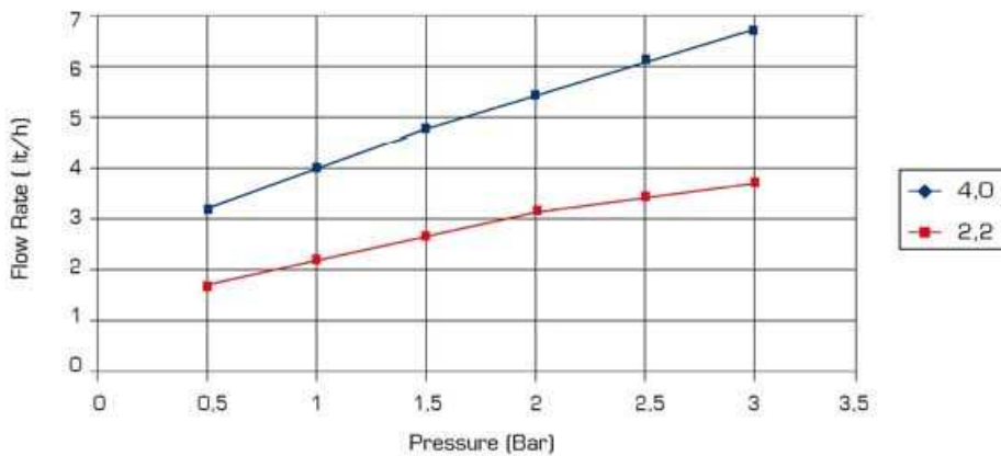
Flow Rate - Pressure Chart
